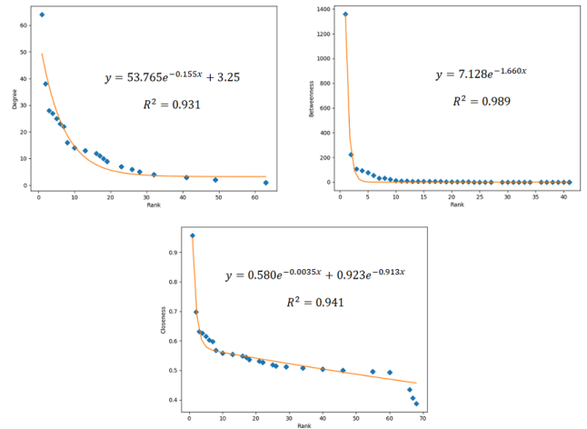
Figure 6. Statistical distributions of degree, betweenness, and closeness.
