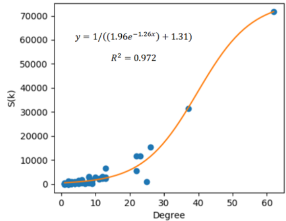
Figure 5. S_k as a function of degree k
