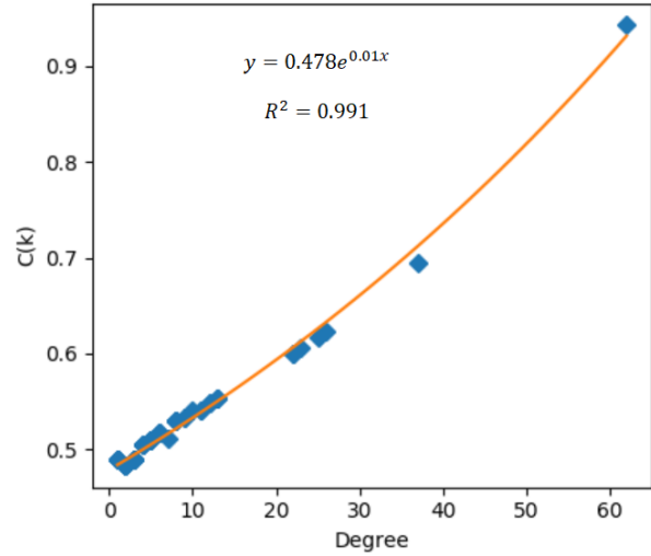
Figure 9. Correlation between the clustering coefficient and degree
