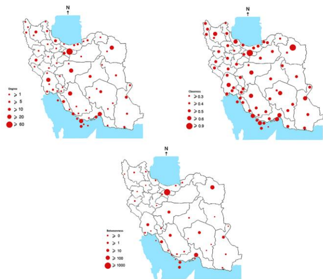
Figure 7. Spatial distributions of degree, closeness, and betweenness.
