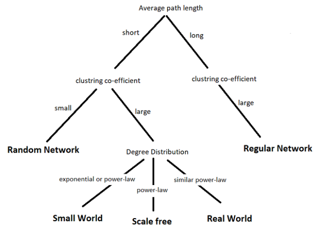
Figure 1. The tree diagram representing the features of different types of networks.
