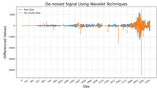
Figure. 5. The denoised signal produced using the wavelet transform approach is shown next to the closing price of the MAPNA stock (post-differentiation).
