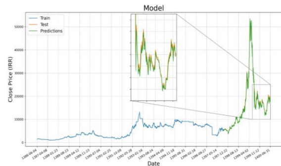
Figure 10. The predicted price chart of MAPNA shares is generated by the CNN-LSTM model.
