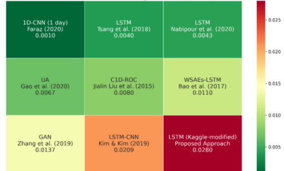
Figure 14. Heat map of MAPE for different papers and our Proposed method.
