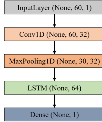
Figure 7. The architecture of the CNN-LSTM model.
